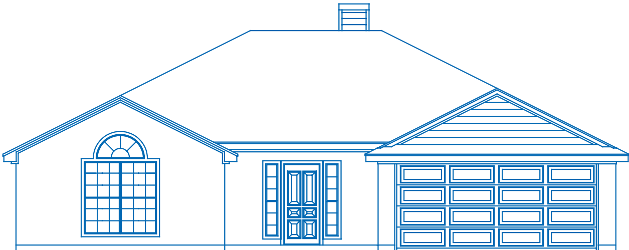
ELEVATION "B"
